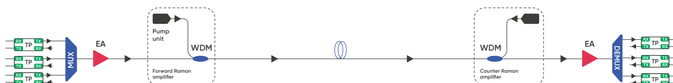
Scheme of a single-span line with erbium and Raman amplifiers
